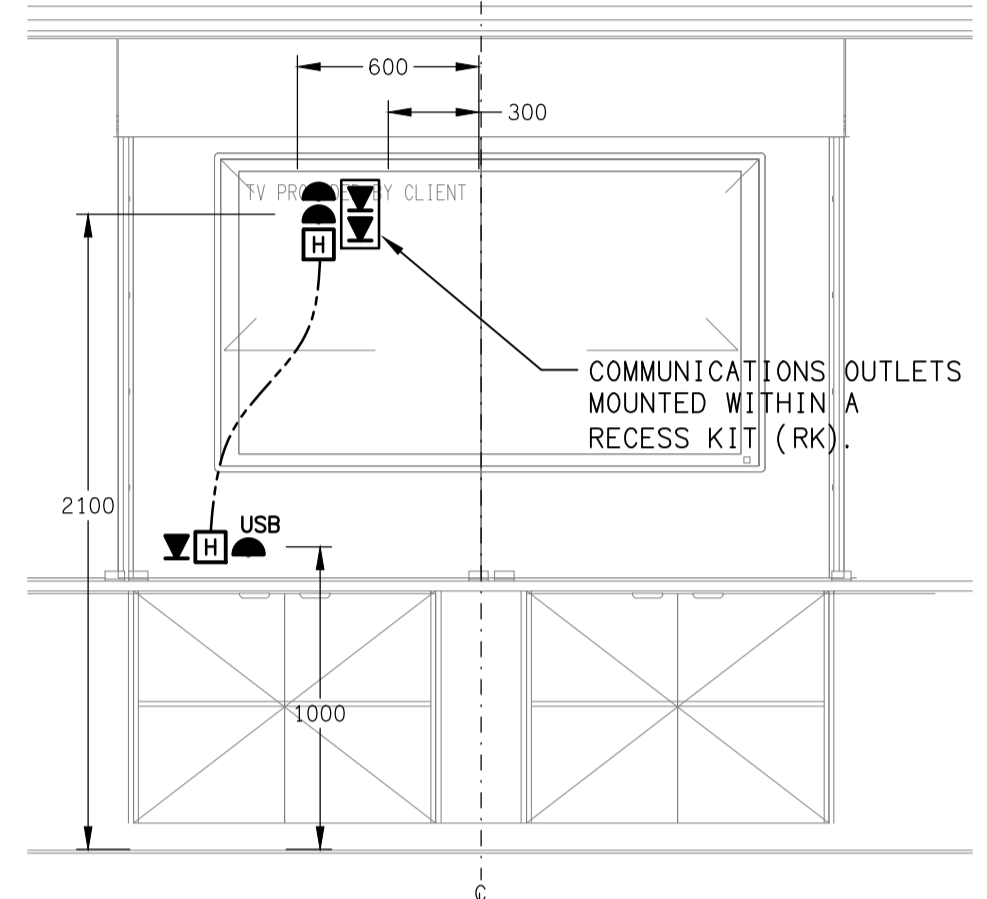
DETAIL C TYPICAL GLA TEACHERS WALL ELEVATION SCALE 1:25
