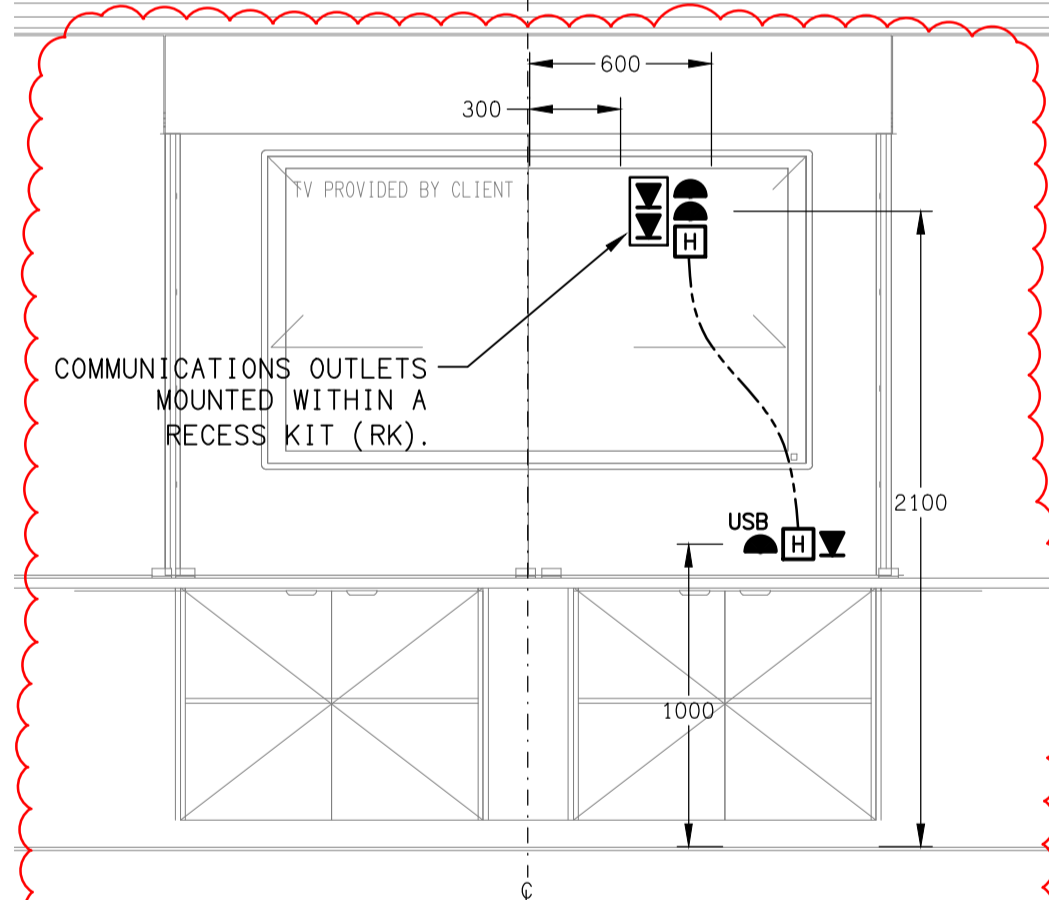
DETAIL D TYPICAL ART STUDIO TEACHERS WALL ELEVATION SCALE 1:25
